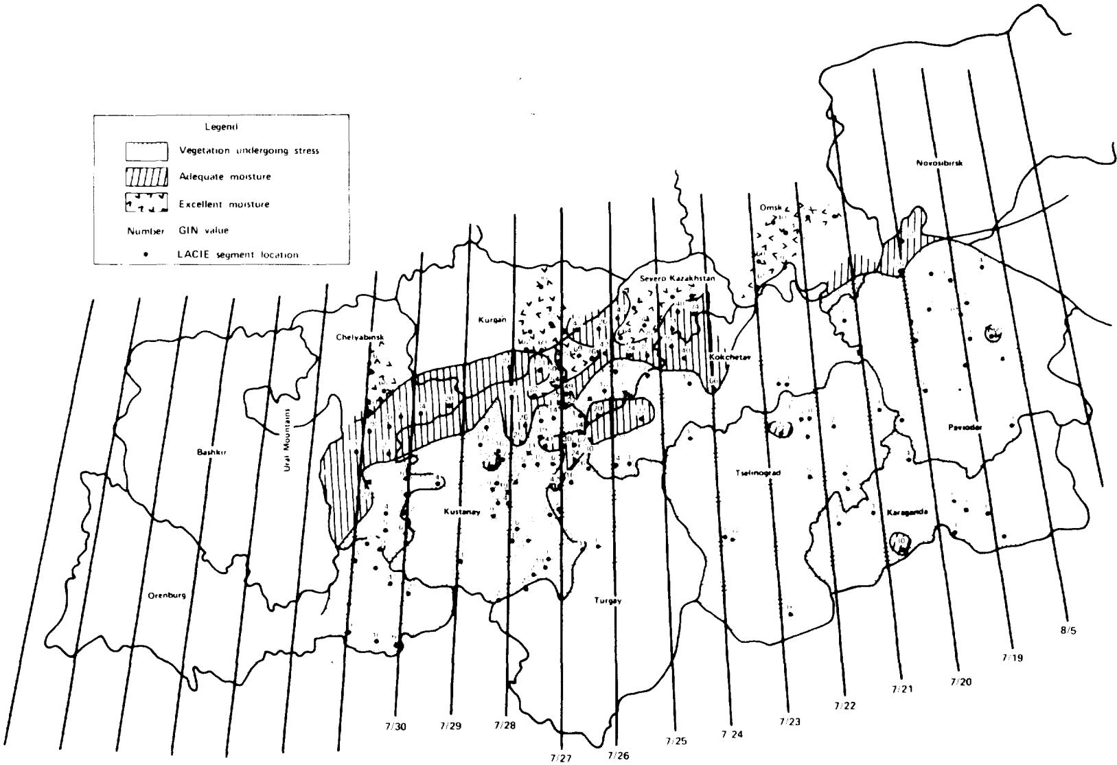
Figure 4. Moisture conditions over USSR spring wheat from the Green Index Number (GIN) monitoring program (Landsat data acquired July 19 through July 30, 1977.)
