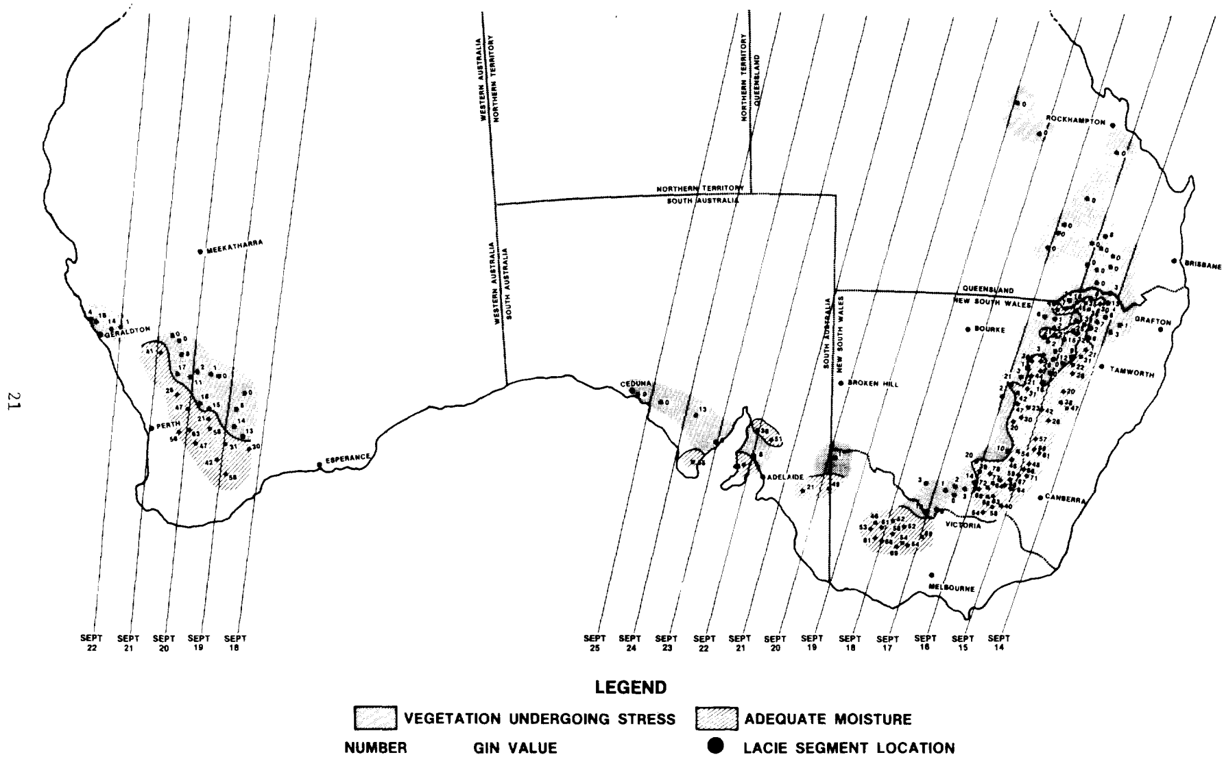
Figure 6. Moisture conditions over Australia wheat from the Green Index Number (GIN) monitoring program for September 14-25, 1977.
