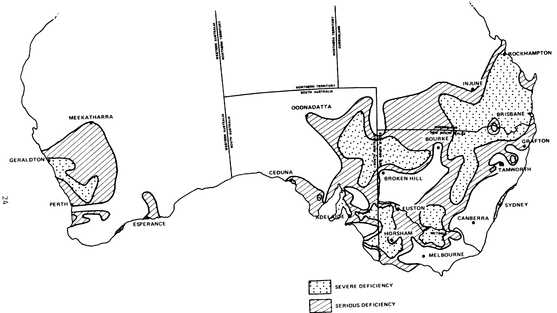
Figure 9. Area of moisture deficiency in Australia as of October 1977 as indicated by rainfall deficiencies.
