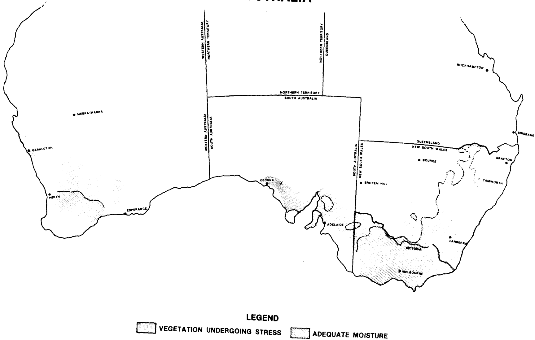
Figure 8. Moisture conditions over Australia wheat from the Green Index Number (GIN) monitoring program for September-October 1977.
