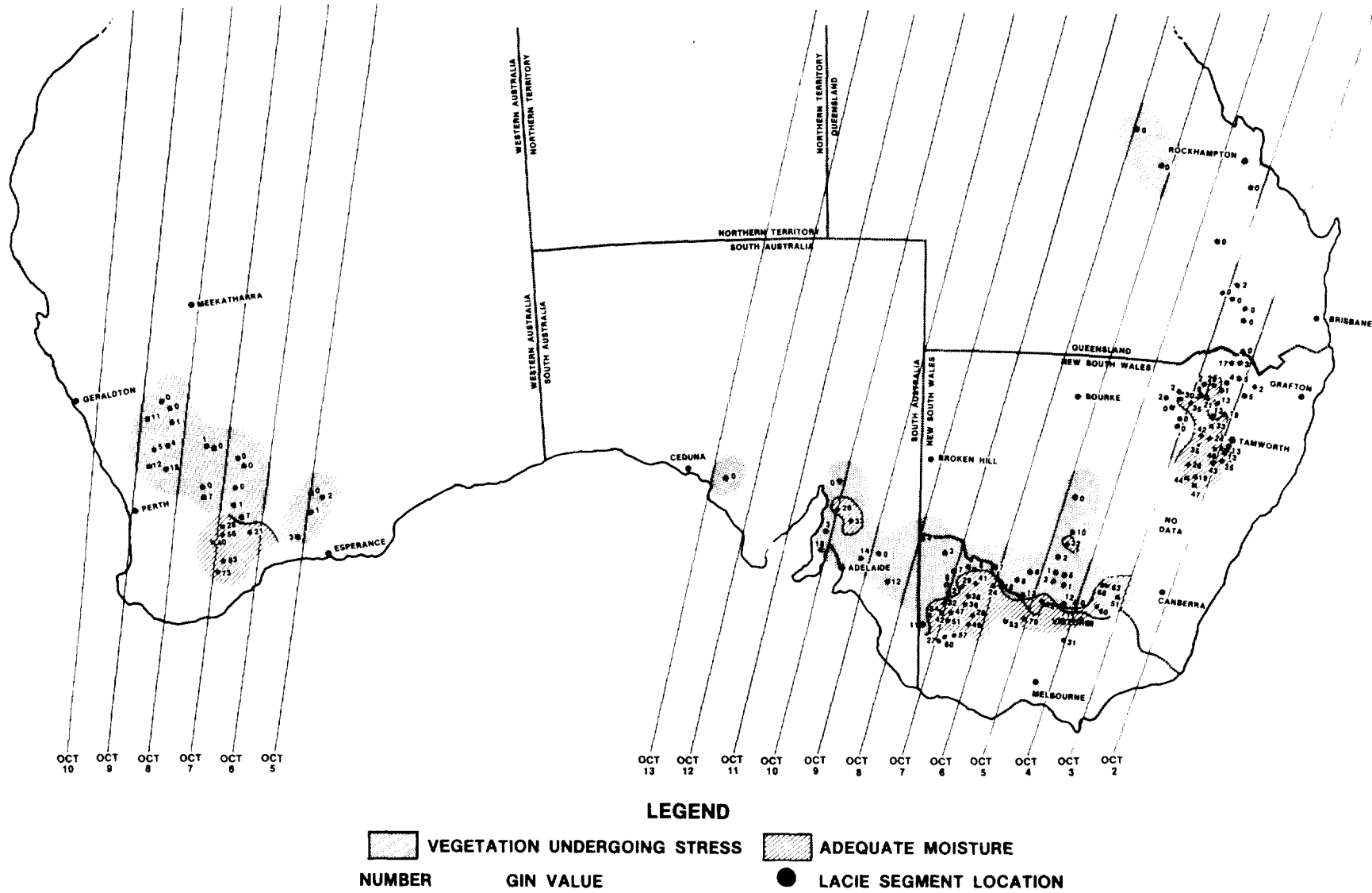
Figure 7. Moisture conditions over Australia wheat from the Green Index Number (GIN) monitoring program for October 2-13, 1977.
