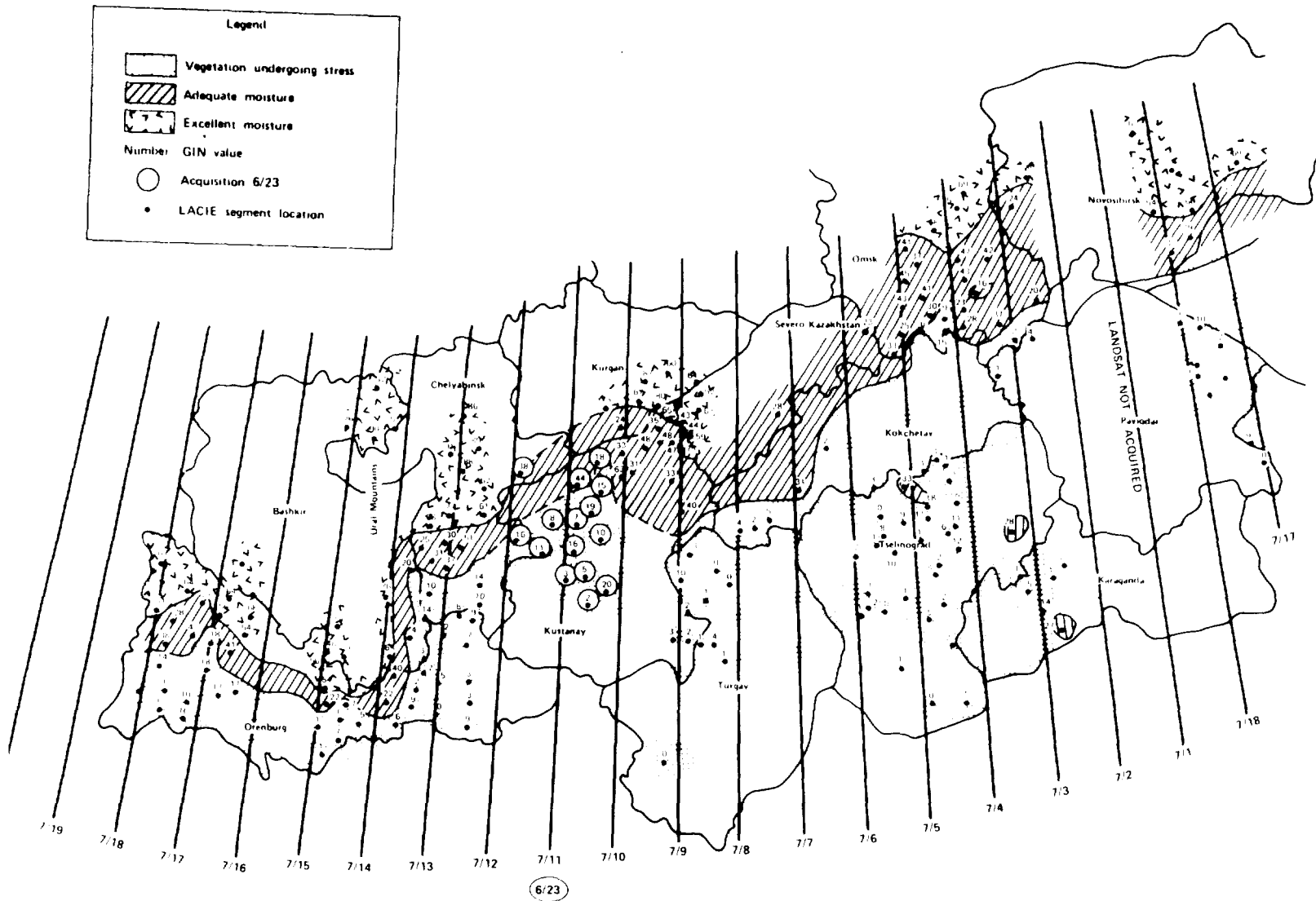
Figure 3. Moisture conditions over USSR spring wheat from the Green Index Number (GIN) monitoring program (Landsat data acquired June 23, 1977, and July 2 through July 19, 1977.)
